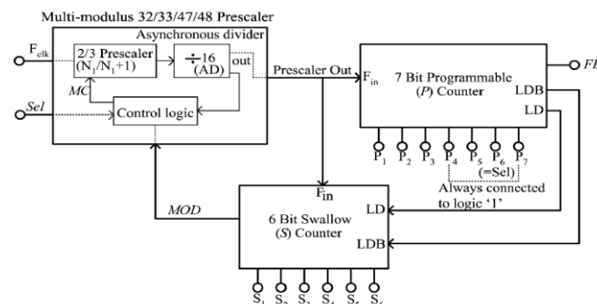
Fig 1: Proposed dynamic logic multiband flexible Divider.
