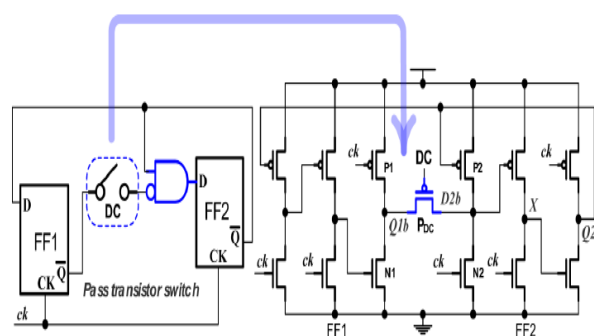
Fig 3: Schematic of proposed E-TSPC based divide-by-2/3 prescaler.
