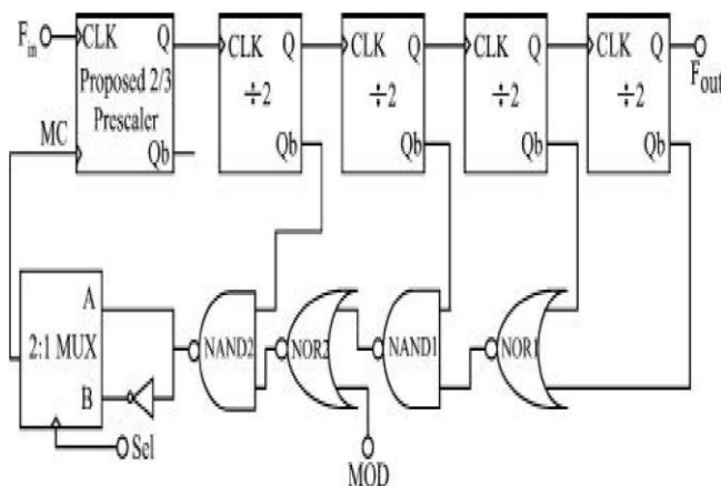
Fig 4: Proposed Multimodulus 32/33/47/48 Prescaler.
