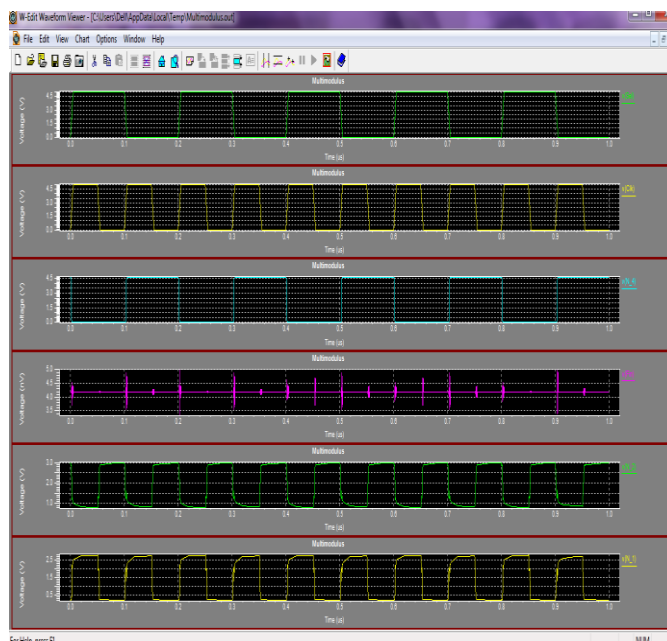
Fig 9: Multimodulus Output Waveform
