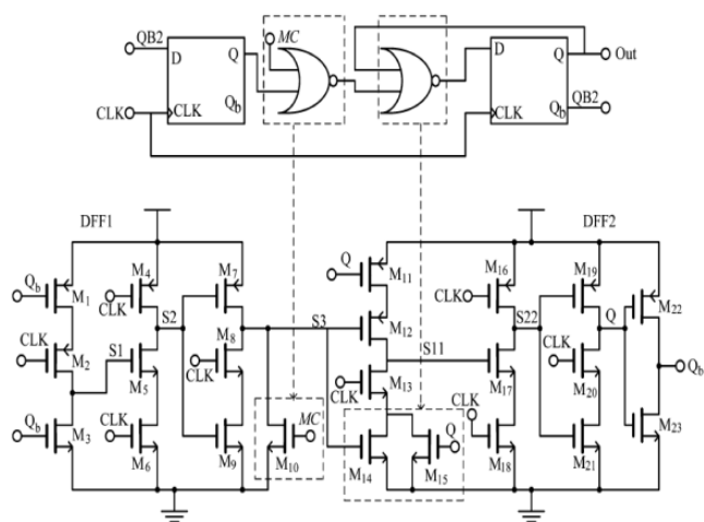
Fig 2: Design-I TSPC 2/3 prescaler circuit and equivalent gate level schematic.
