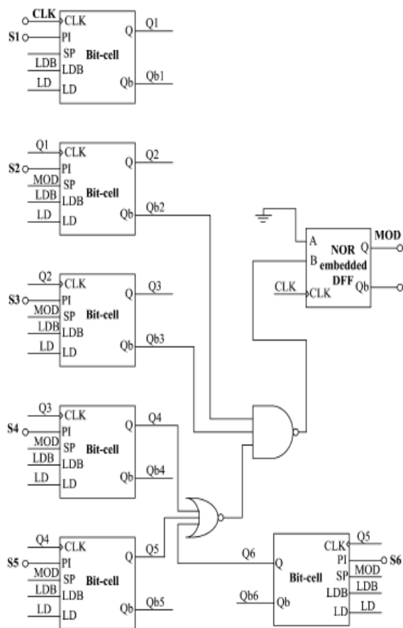
Fig 5: Asynchronous 6-Bit S-Counter.
